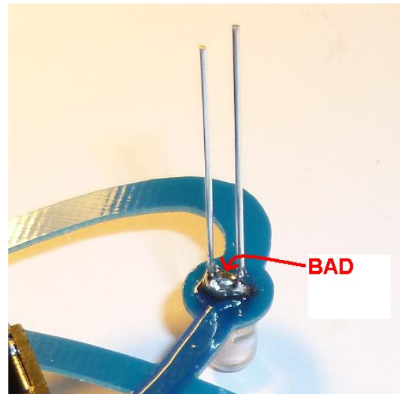
A bridge between the two leads of the LED. Current will flow through the bridge, and not the LED, thus the LED will not light up. Fortunately, this is easy to fix.
